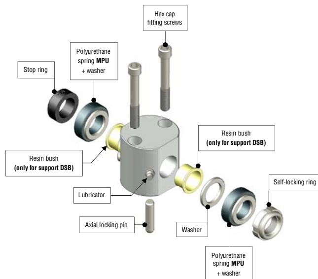
DBB/DNB/DSB supports - exploded diagram
