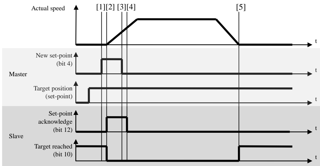
&lt;Set-point example&gt;
