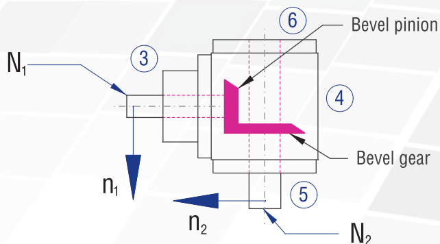
Figure 6.3.3-2; Shaft designations
